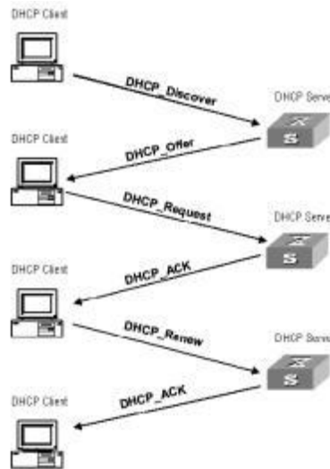
Figure 2-1. Interaction process
